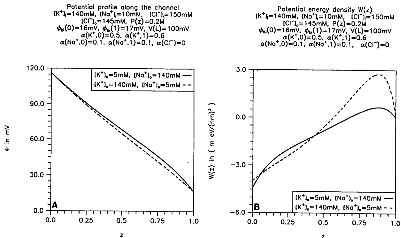
FIGURE 4 (A) The electrical potential \Phi(z) under two different ionic conditions. The conditions are specified in the figure itself, the text, and Table 3. The difference in potential seems small to the eye, but it appears in integrals of exponential functions of the potential and so it has a significant effect on the concentration C_i(z) and the flux, particularly its qualitative properties shown in Fig. 3. Coupling occurs in the PNP model because the change in bathing concentrations changes the distribution of potential \Phi_m(z) . (B) The energy density W(z) under two different ionic conditions. W(z) measures the potential energy of the concentration of all ions z_i C_i(z) at that location; it determines the macroscopic flux J_i more directly than the electrical potential \Phi(z) and so, not surprisingly, changes more dramatically than \Phi(z) when ionic concentrations are changed (as specified in the figure itself, the text, and Table 3).
